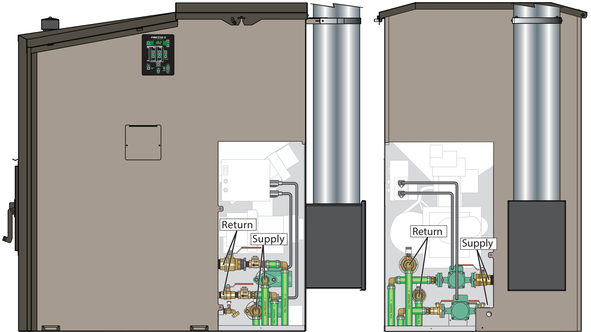
Side View
